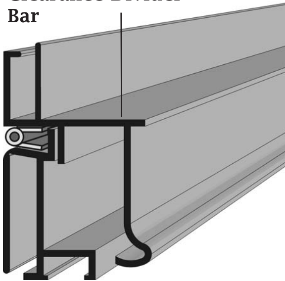
Heavy Duty Zero Clearance Carrier
